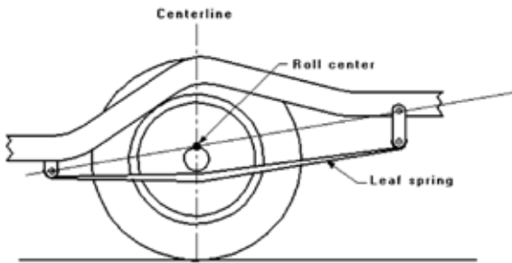
FIGURE 16: HOTCHKISS REAR AXLE
